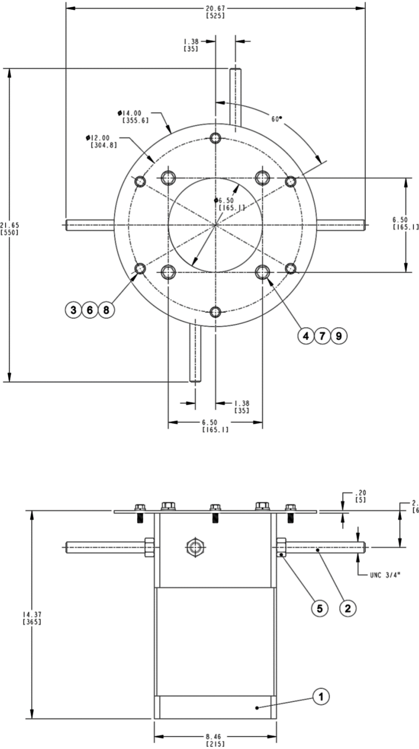
Fig.1 – Top & front view
