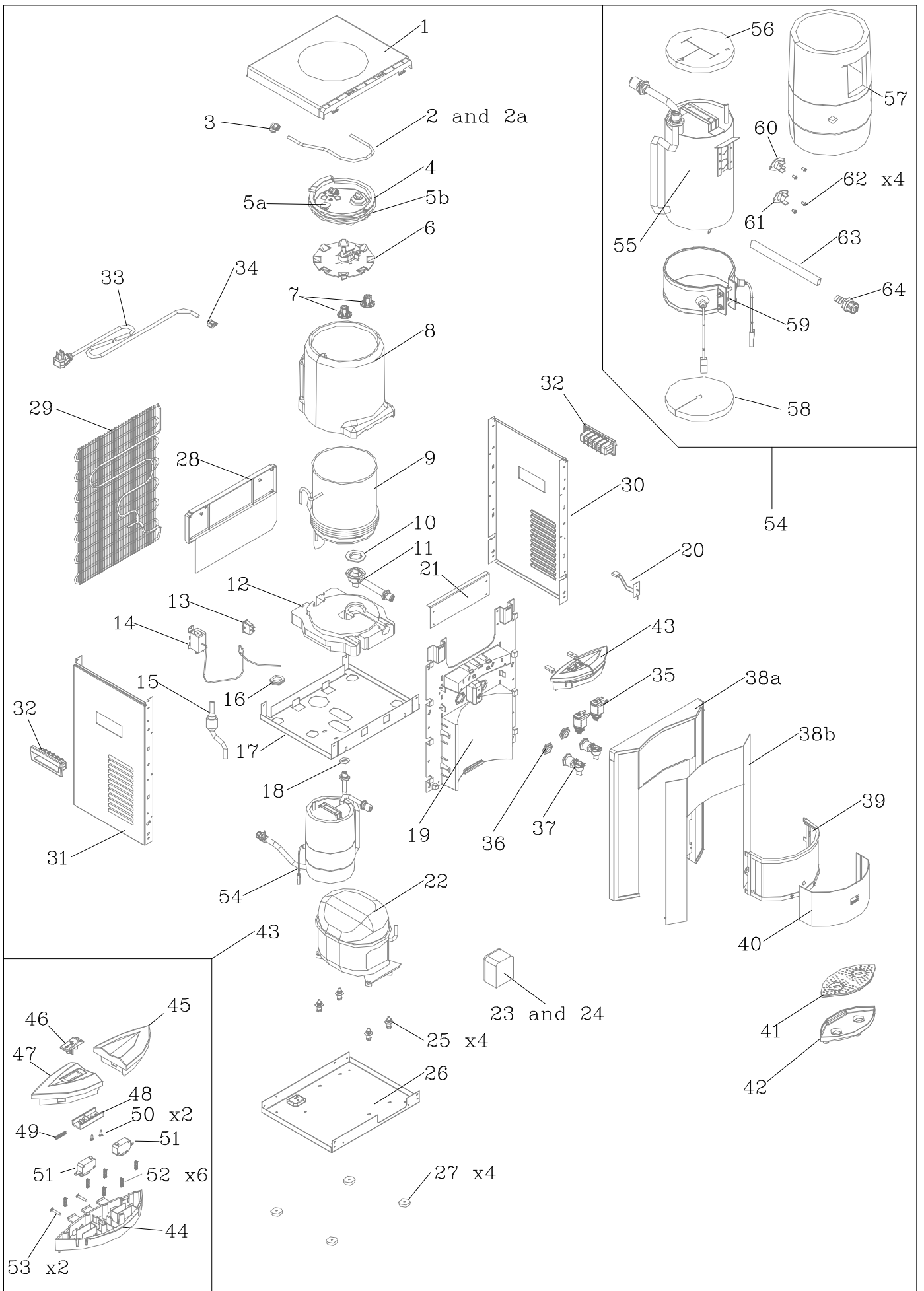
POU1CCT Model Cooler
